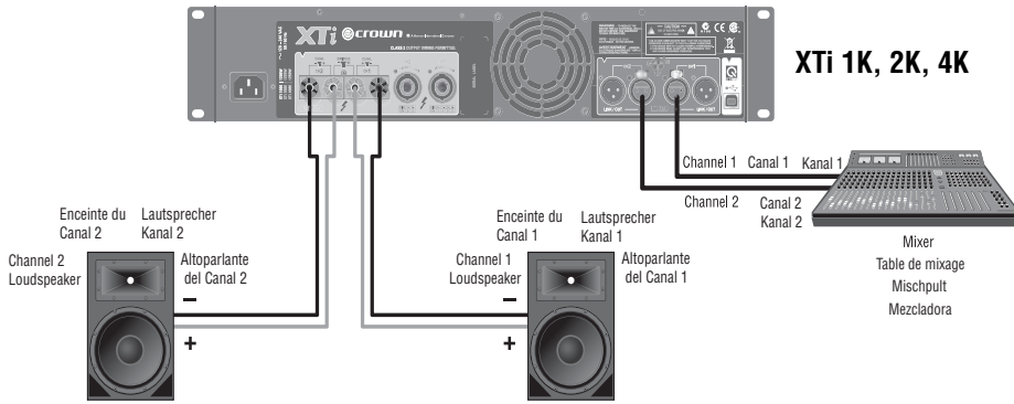
Figure 2.6 System Wiring, Stereo Mode Using the Binding Posts
